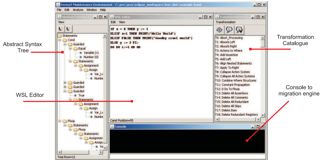
Figure 2: Components of the FermaT Maintenance Environment
