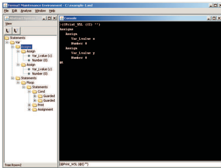
Figure 9: Console to the transformation engine
