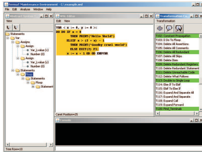
Figure 8: Transformation Example
