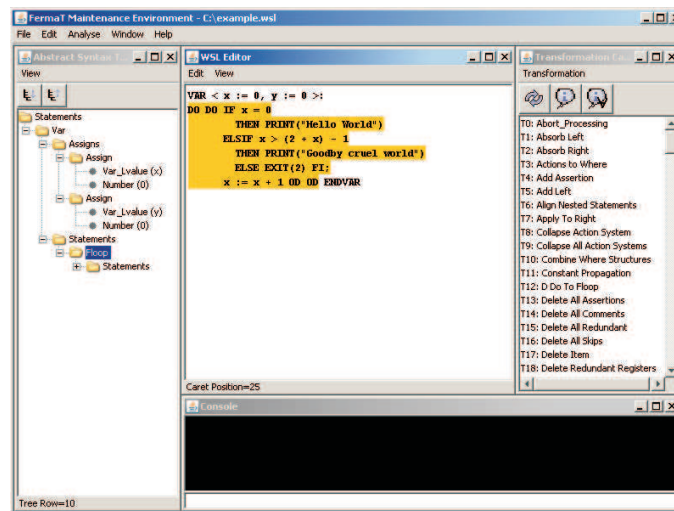
Figure 6: Transformation Example
