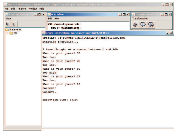
Figure 5: Execution of the guessing game
