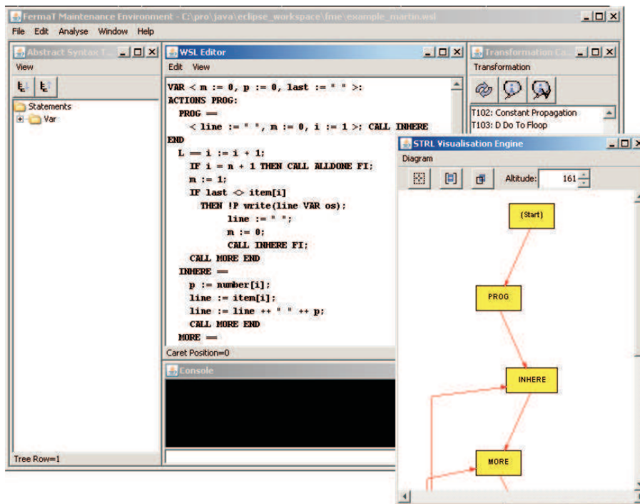
Figure 10: ActionSystem CallGraph
